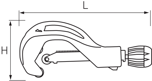
ANK0040, 20 mm - 63 mm (3/4" to 2½") Pipe Cutter, uses replacement blades ANK0240.
