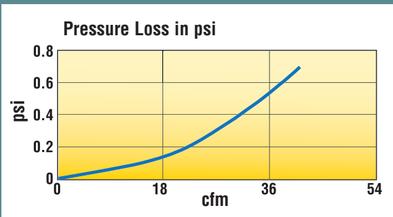
Pressure Loss in Couplers
